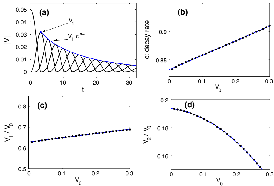
Fig. 6 Illustration of the procedure to obtain the scaling law for the decay of the velocity profile. This example is for strike and observation on the 30^\circ line. a Magnitude of velocity of beads 0–12 versus time in the ideal parameter case with V_0 = 0.05 . The maxima are fit with a function of the form V_1 c^{n-1} , where V_1 is the maximum velocity of the first bead (labeled in the plot). This processes is repeated for several values of V_0 to obtain a sequence of decay rates c(V_0) . b The sequence
