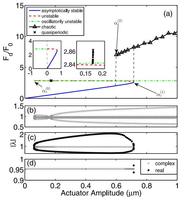
Fig. 2: (Color online) (a) Numerical bifurcation diagram of average dynamical force at the fourth site of the chain normalized against the static load F_0 , continued as a function of actuator amplitude. The three time-periodic branches are shown by the lines without markers. Past \alpha = \alpha_c^{(2)} , an additional chaotic branch also exists, denoted by the line with triangle markers. A Hopf bifurcation that spawns a branch of quasiperiodic solutions is shown by an “x” marker. An enlarged view of the Hopf bifurcation is shown in the right inset. The left inset shows the corresponding bifurcation diagram for the undamped system, where the unstable branch reaches \alpha = 0 \mu\text{m} and extends towards the oscillatorily unstable branch for \alpha < 0 . The bottom three panels show the moduli of the Floquet multipliers for the oscillatorily unstable dash-dotted branch (b), the unstable dashed branch (c), and the stable solid branch (d).
