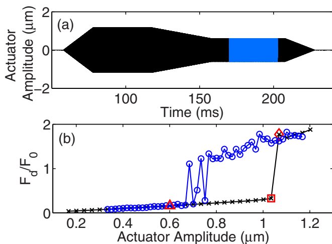
Fig. 6: (Color online) (a) The hysteresis loop driving amplitude for the run marked by the red triangle in (b). The initial driving amplitude is 1.2 \mu\text{m} for all experiments. The blue region highlights the time interval over which the PSD was calculated. (b) Experimentally characterized hysteresis loop showing dynamic force as a function of actuator driving amplitude, at a driving frequency of 6 kHz. Black “x” markers denote following the stable periodic solution to chaos, while blue circles denote the return from a chaotic response back to the low-amplitude periodic response. The red square and diamond markers correspond to the blue square and diamond, respectively, of fig. 5(a).
