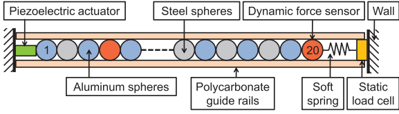
Fig. 1: (Color online) Schematic of the experimental setup.
