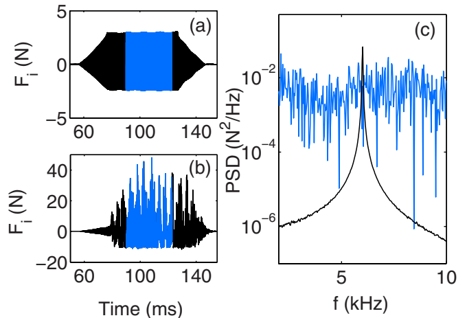
Fig. 4: (Color online) Experimental force-time histories measured by the sensor at n = 4 , corresponding to (a) the largest low-amplitude periodic response (blue square in fig. 5), and (b) the first amplitude following the onset of chaos (blue diamond in fig. 5). The central blue region highlights the time interval over which the PSD was calculated. (c) The black and blue curves are the PSD of the signals in (a) and (b), respectively.
