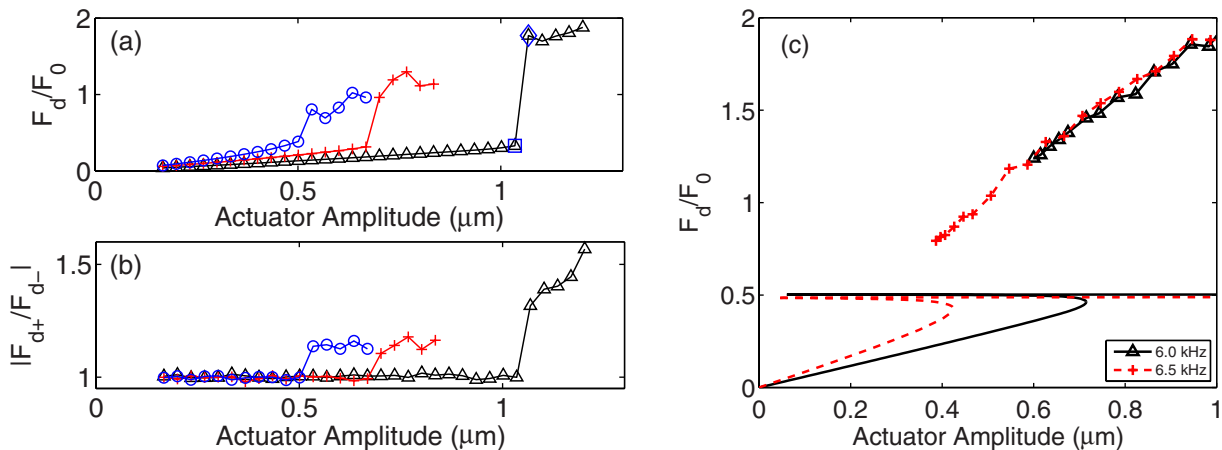
Fig. 5: (Color online) (a) Dynamic force amplitude at driving frequencies of 6 kHz (black triangles), 6.5 kHz (red crosses), and 6.8 kHz (blue circles). The blue square corresponds to the force-time history immediately before the onset of chaos (fig. 4(a)), while the blue diamond corresponds to the force-time history immediately following the onset of chaos (fig. 4(b)). (b) Asymmetry of the force-time response, as the actuator displacement is increased. The onset of asymmetry (as |F_{d+}/F_{d-}| becomes > 1 ) corresponds to the onset of instability for all three driving frequencies. (c) Numerically obtained dynamic force amplitude at driving frequencies of 6 kHz (black solid line with triangles) and 6.5 kHz (red dashed line with crosses). In each case, lines without markers are numerically exact periodic solutions, while the lines with markers are the chaotic branches.
