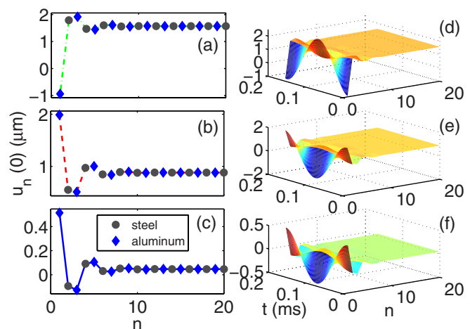
Fig. 3: (Color online) Sample profiles at t = 0 (left panels) and spatiotemporal evolution of the solutions (right panels) for each of the three breather branches are shown for \alpha = 0.4 \mu\text{m} . Panels (a), (d) correspond to the oscillatorily unstable dash-dotted branch; (b), (e) to the unstable dashed branch, and (c), (f) to the stable solid branch.
