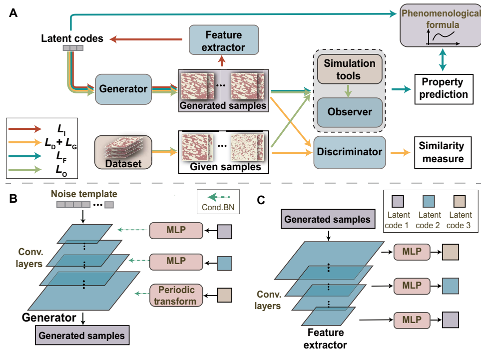
Fig. 2. Detailed network architectures of the GNMD. (A) Illustration of the workflow of GNMD. The flow of information for calculating different losses is represented by different colored arrows. The red arrows represent the workflow for maximizing mutual information to extract a parameterization of relevant geometric features for expected material properties. The yellow arrows represent the classic WGAN-GP (40) workflow, optimizing the generator and discriminator to generate realistic samples. The bottle green arrows demonstrate the fitting-loss workflow, aiming to establish the relationship between material properties and extract principal geometric features that determine bulk material properties. The pale green arrows illustrate the optimization workflow for the observer. (B) Latent code input mechanism in the generator for a three-parameter case. The input latent code is fed into the network from various layers using conditional batch normalization, implemented either via a fully connected layer or periodic transformation (in the case of periodic latent code). BN, batch normalization; MLP, multilayer perceptron. (C) Latent code information output mechanism in the feature extractor for a three-parameter case. Combined with the position of the latent code input layer, the latent code information is restored through the fully connected layers, which followed by the corresponding layers of the CNN network.
