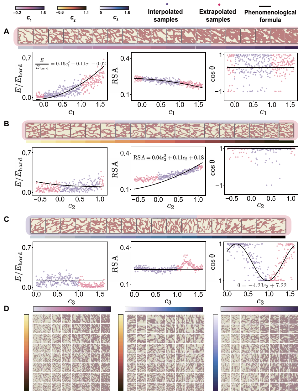
Fig. 4. Geometric feature extraction and inverse design considering three different material properties concurrently. The samples are generated with gradually changing interpolated and extrapolated latent codes. The maximum Young's modulus (normalized by E_{\text{hard}} , the Young's modulus of the hard material), RSA (the relative surface area), and \theta (the orientation of the maximum modulus) of these samples are calculated by the physical module and predicted by the phenomenological formula. (A) Results for varying c_1 and fixed c_2 = 0.47 and c_3 = 0.52 . (B) Results for varying c_2 and fixed c_1 = 0.63 and c_3 = 0.19 . (C) Results for varying c_3 and fixed c_1 = 0.69 and c_2 = 0.56 . (D) Latent-space atlas of generated microstructures. Representative microstructures sampled by sweeping pairs of latent coordinates ( c_1, c_2, c_3 ). Each grid shows a 2D slice through the 3D latent space with the remaining coordinate held fixed at its median value: left, c_1 - c_2 ; middle, c_2 - c_3 ; right, c_1 - c_3 . Color bars indicate the value ranges of each coordinate.
