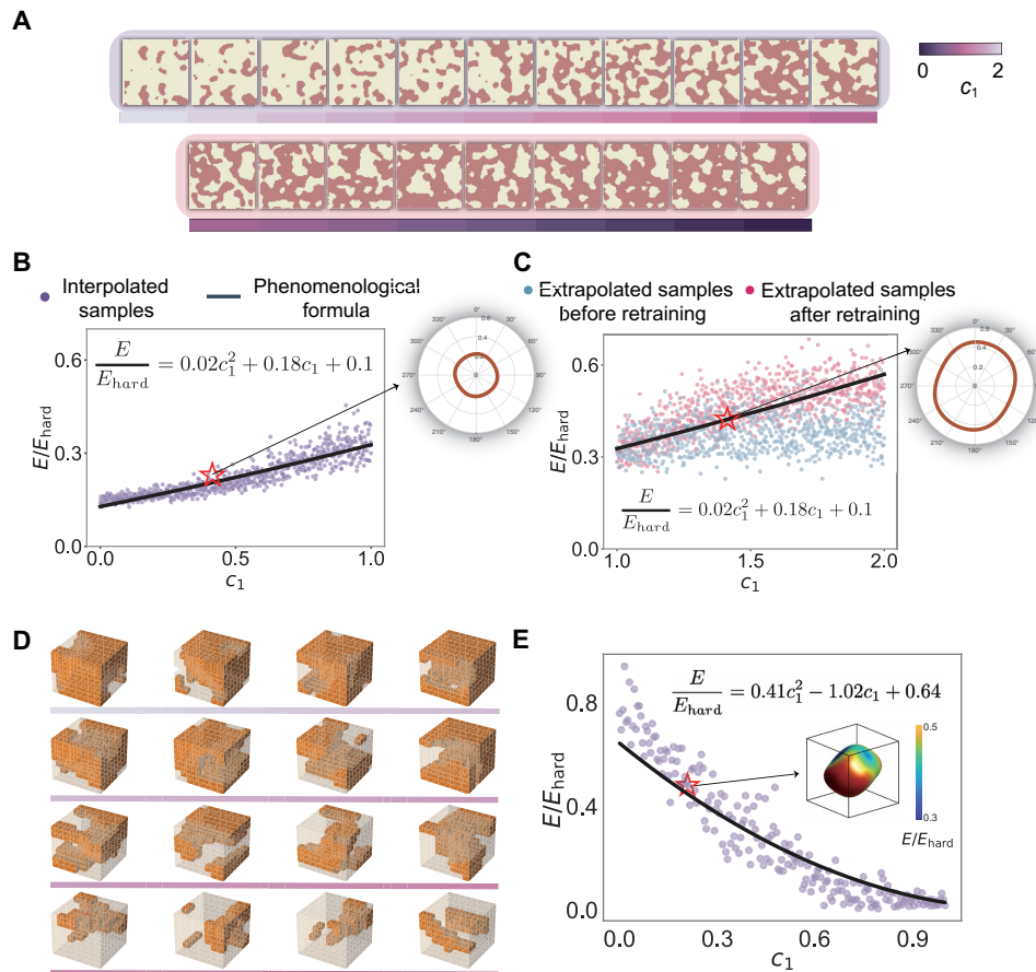
Fig. 3. Examples in 2D and 3D for a single pair of material property and geometric feature. (A) Generated 2D samples with random noise templates and gradual changes in latent codes. (B) Comparison between the Young's moduli (normalized by E_{\text{hard}} , the Young's modulus of the hard material) predicted by the phenomenological formula and FEM for generated interpolated samples within the range of the given dataset. This includes results of the directional Young's modulus at a typical point. (C) Comparison between the elastic moduli predicted by the phenomenological formula and FEM for the generated extrapolated samples before and after retraining outside the range of the given dataset, including results of the directional Young's modulus at a typical point. (D) 3D generated materials with gradual modifications in latent codes. (E) Comparison between the elastic moduli predicted by the phenomenological formula and FEM, including the directional Young's modulus at a selected point.
